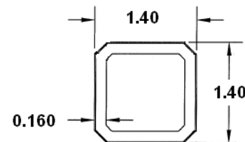
Figure 2 Baluster Profile
